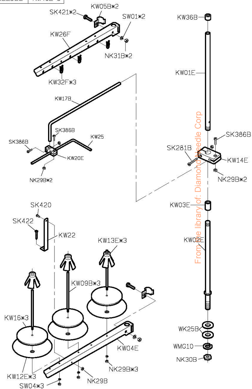
PARTS LIST FOR THREAD STAND GROUP
