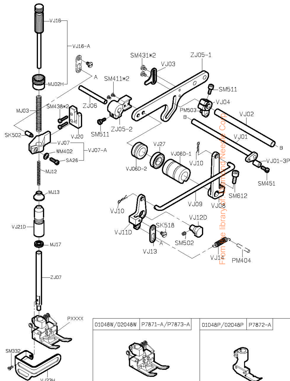
PARTS LIST FOR ZJ GROUP
