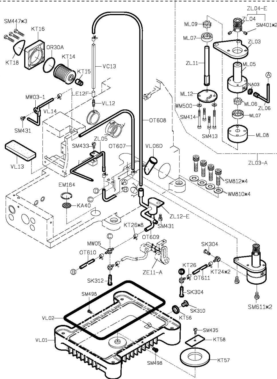
PARTS LIST FOR ZL GROUP
