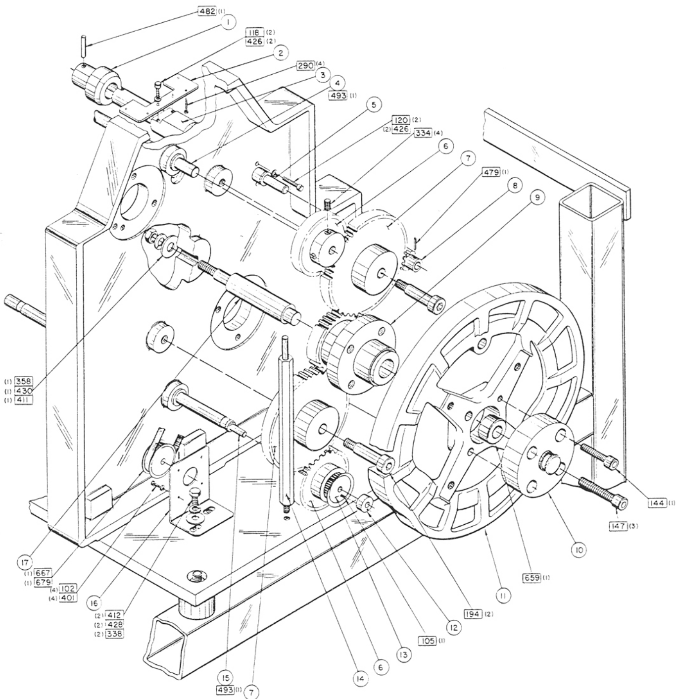
84-4 BUTTON STITCHING MACHINE GEAR TRAIN ASSEMBLY E B S
