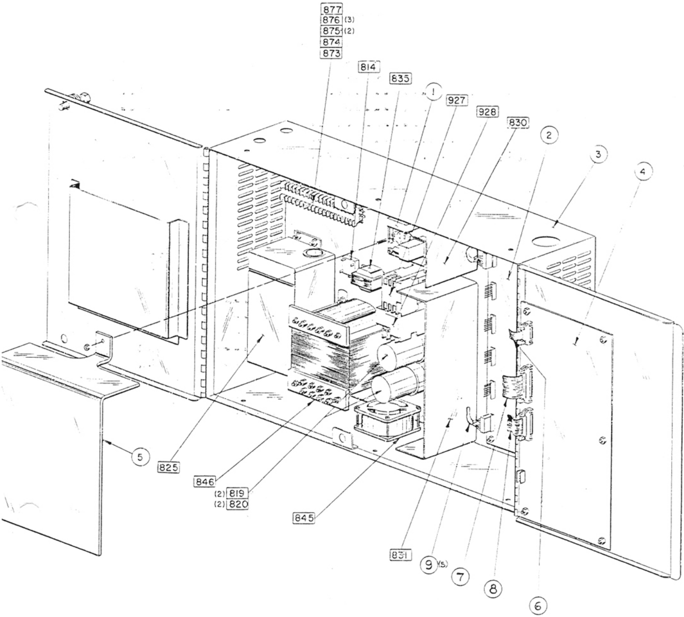
84-4 BUTTON STITCHING MACHINE CONTROL BOX ASSEMBLY 41651-138 E.B.S.
