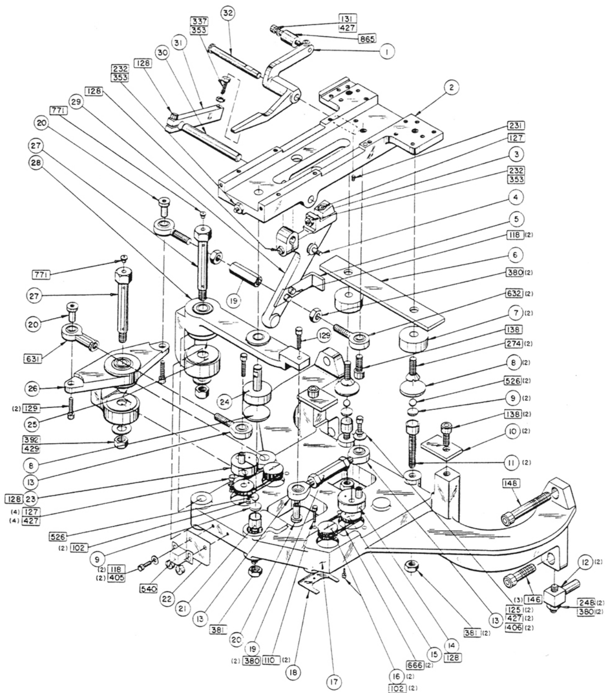
84-4 BUTTON STITCHING MACHINE LOWER TABLE MECHANISM E. B. S.
