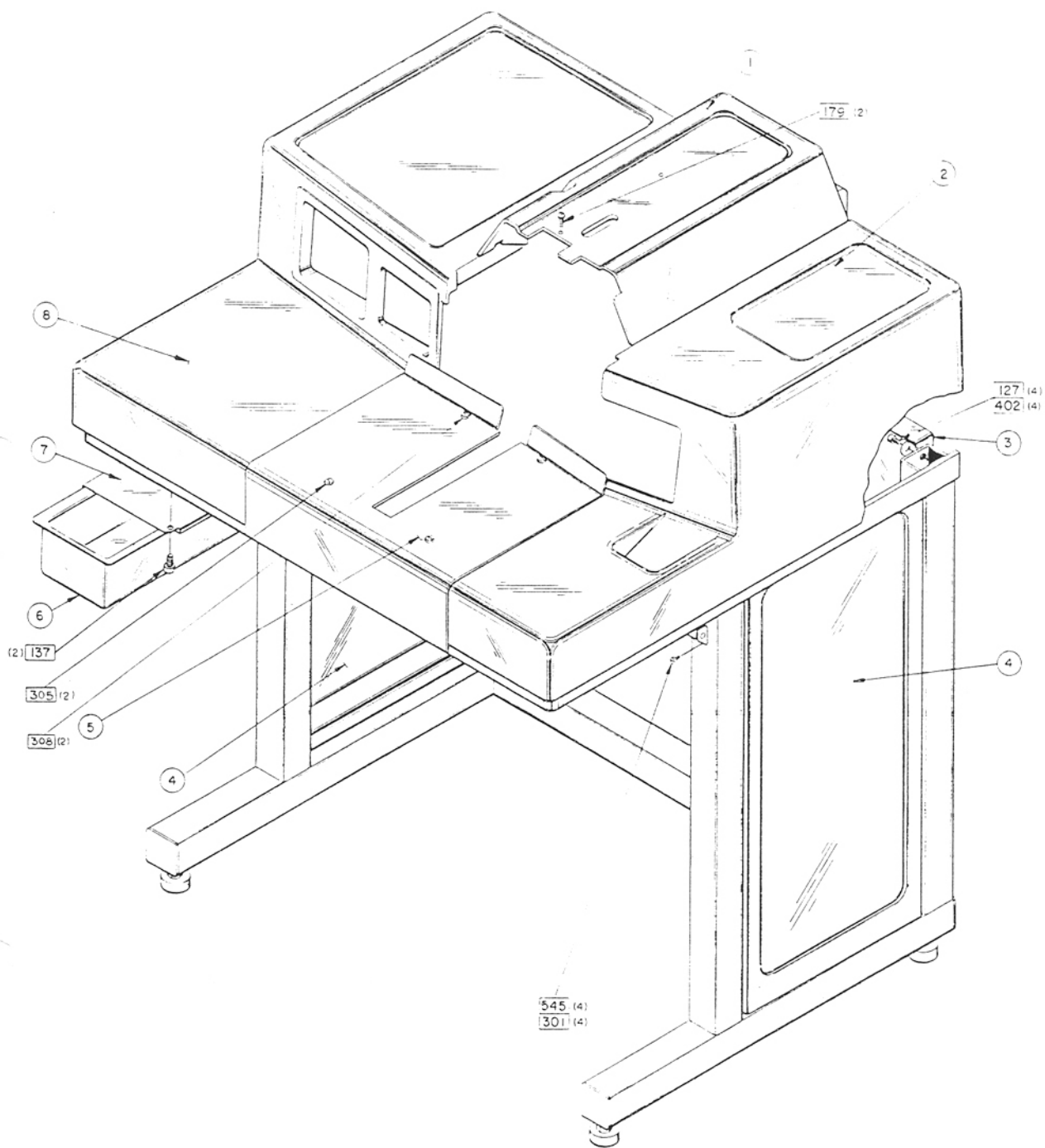
84-4 BUTTON STITCHING MACHINE COVERS & GUARDS ASSEMBLY E B S
