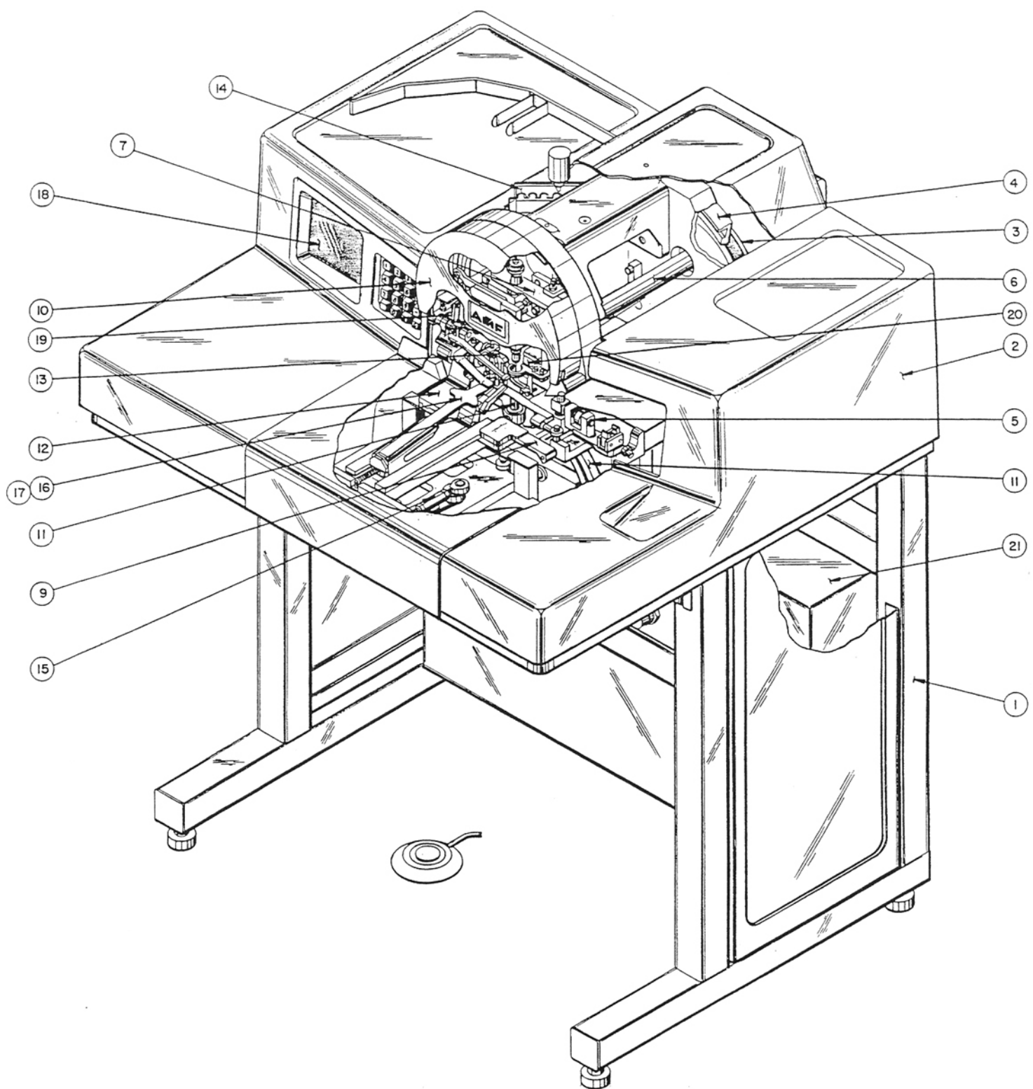
84-4 BUTTON STITCHING MACHINE GENERAL ASSEMBLY 49965-215 E.B.S.
