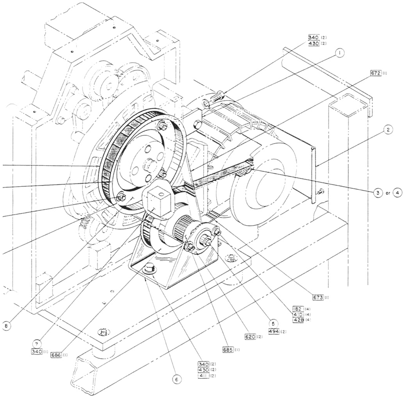
84-4 BUTTON STITCHING MACHINE BELT DRIVE/MOTOR ASSEMBLY E.B.S.
