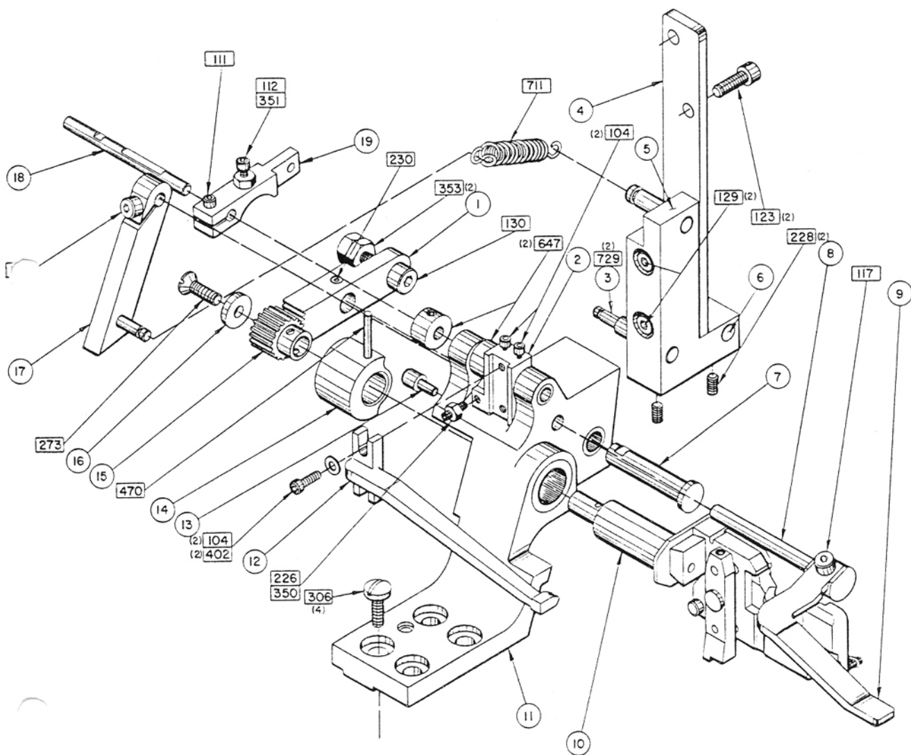
84-4 BUTTON STITCHING MACHINE BUTTON CHUCK MECHANISM 44820-001 E.B.S.
