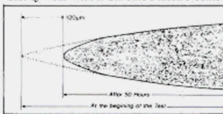
Test of Wear with a Chrome Plated Needle
