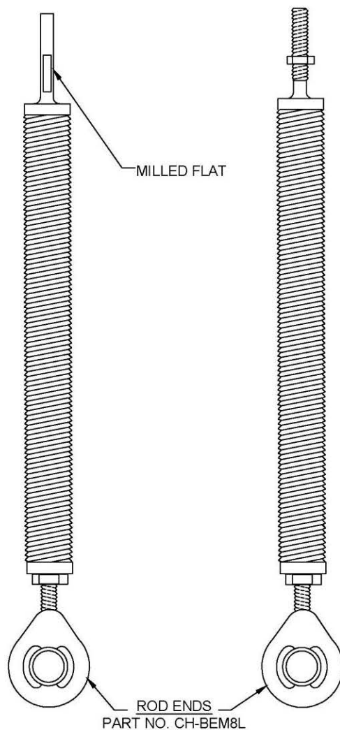
FRONT SUPPORT SPRING PART NO. CH-38-SF
