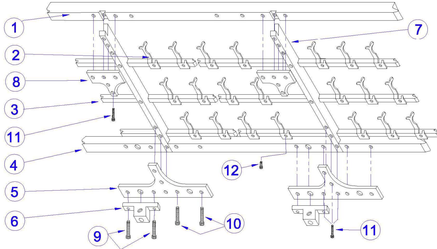
CENTER SECTION OF SPREADER FRAME LOOKING FROM REAR OF MACHINE
