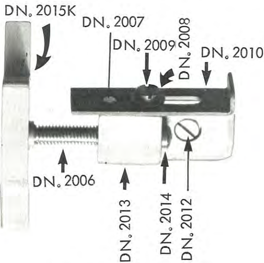
DN.2005K signature stop complete
