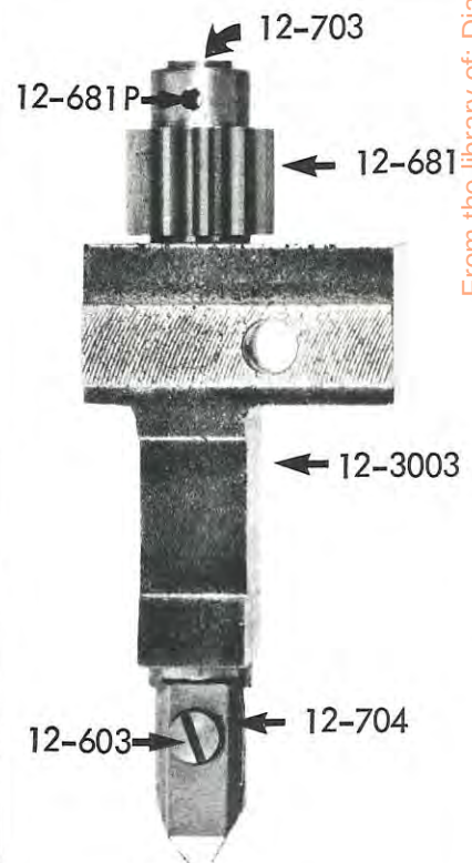
12-703K Hook Revolving Mechanism complete with hook block (contains 12-603, 12-681, 12-681P, 12-703, 12-704, 12-3003)
