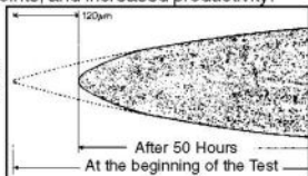
Test of Wear with the Chrome Plated Needle
